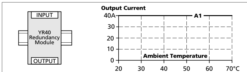
Fig. 19-3 Mounting Orientation A (Standard orientation)
