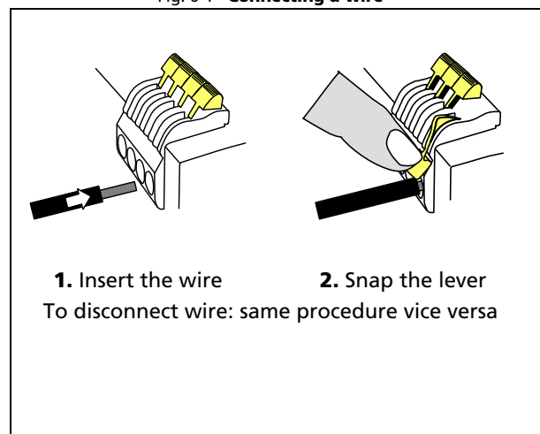
Fig. 6-1 Connecting a wire
